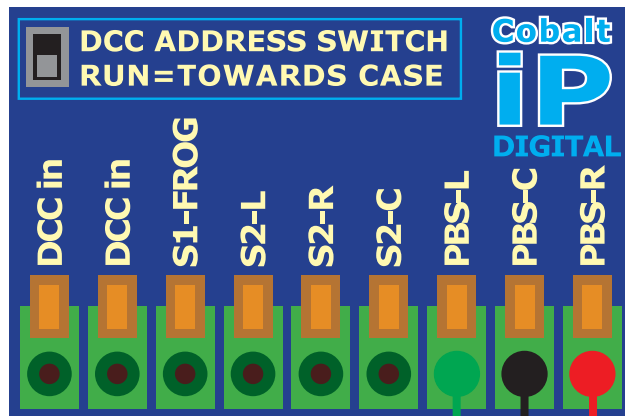
Cobalt iP Digital Point Motor DCC-CB1DIP
