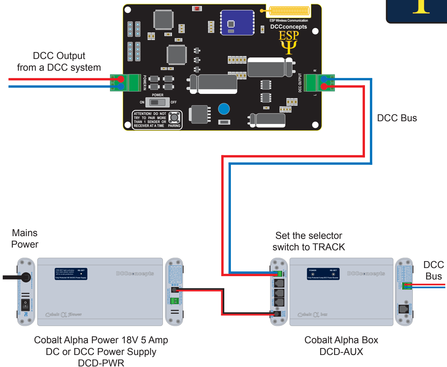
ESP Wireless DCC Receiver Unit DCC-ESPR.1
