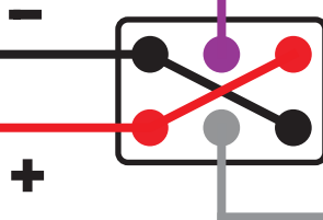
Double Pole Double Throw DPDT Toggle Switch
