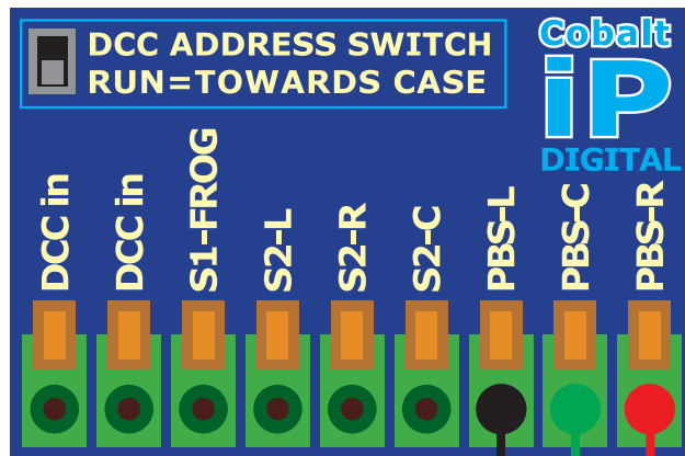
Cobalt iP Digital Point Motor DCP-CB1DIP
